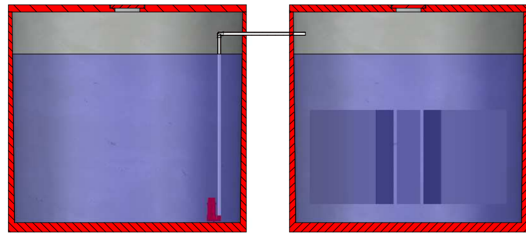
SECTION B-B
